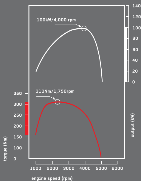
2.0 litre Diesel engine
